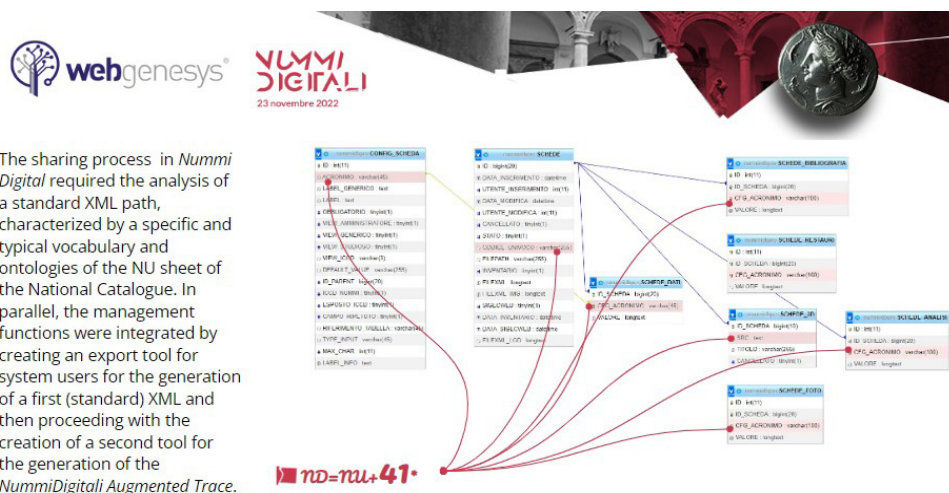
Fig. 8. Synoptic NU – NU+ and LOD.
